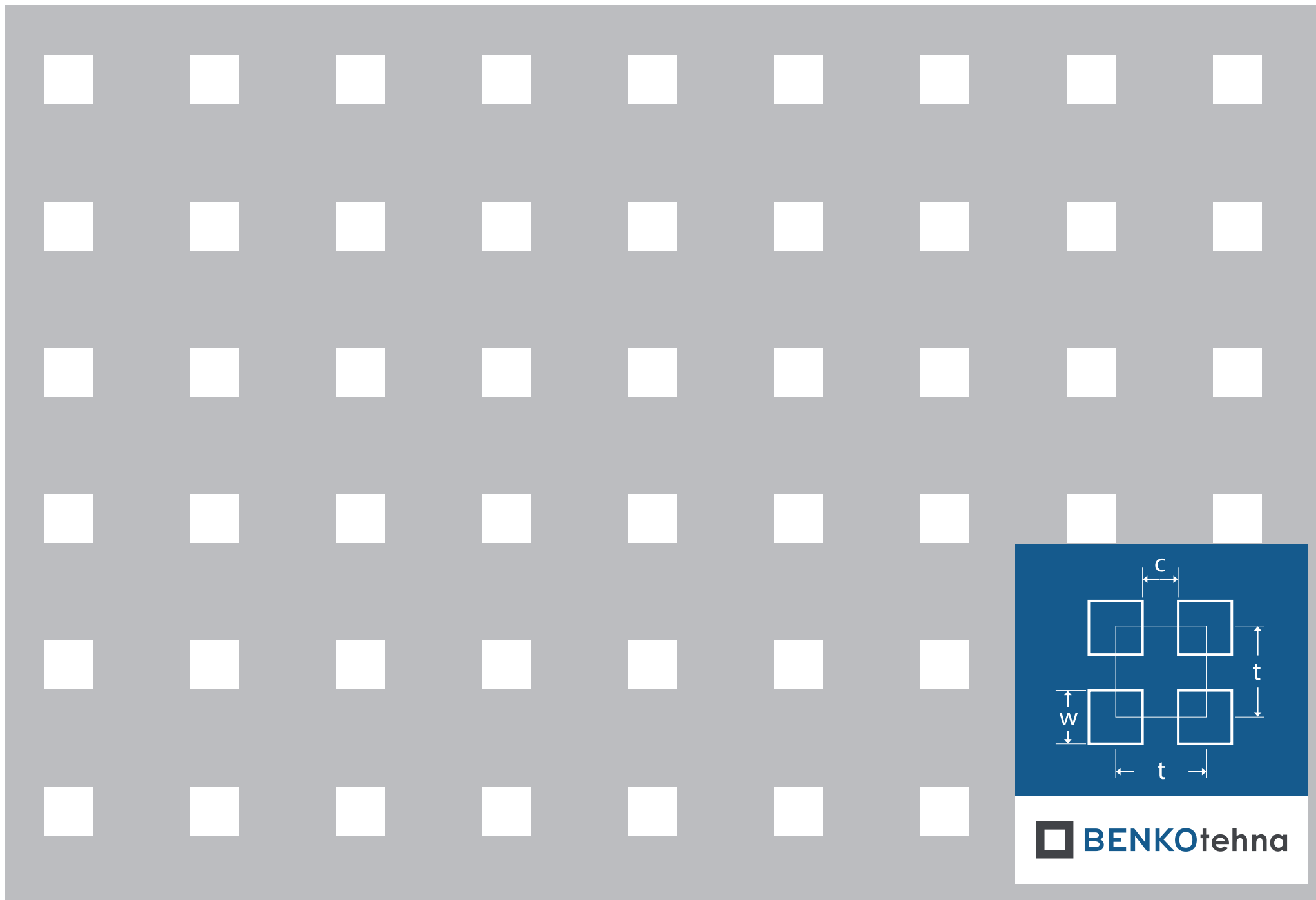
Kvadratna redna Kr 10-30: w = 10,0 \text{ mm} | c = 20,0 \text{ mm} | t = 30,0 \text{ mm} | otvorenost = 11,11%
