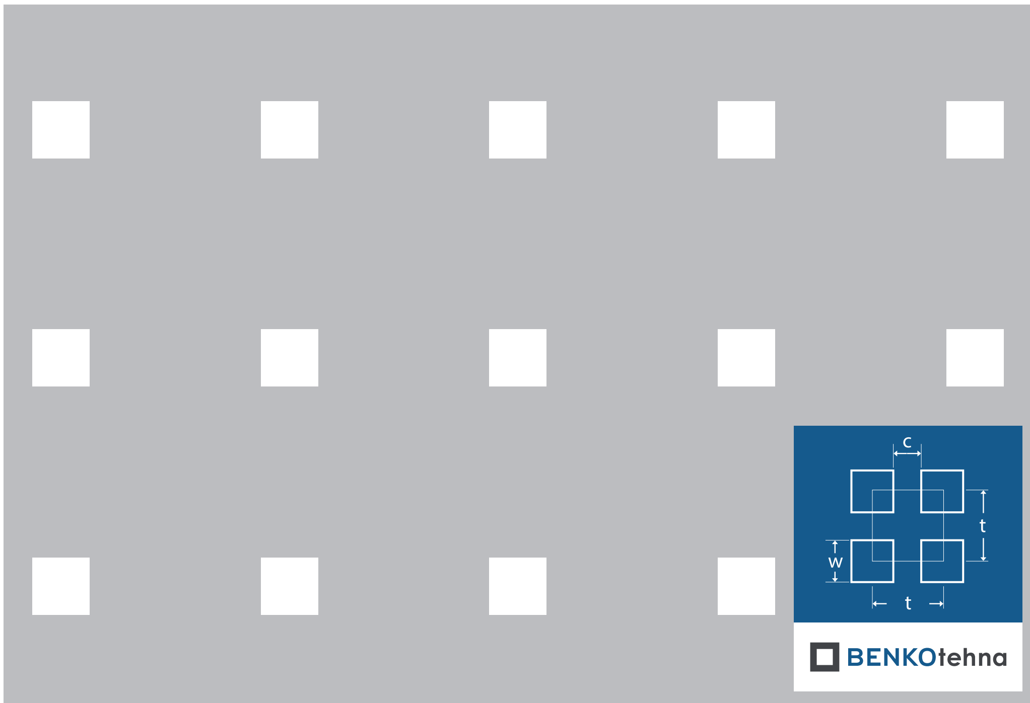
Kvadratna redna Kr 15-60: w = 15,0 \text{ mm} | c = 45,0 \text{ mm} | t = 60,0 \text{ mm} | otvorenost = 6,25%
