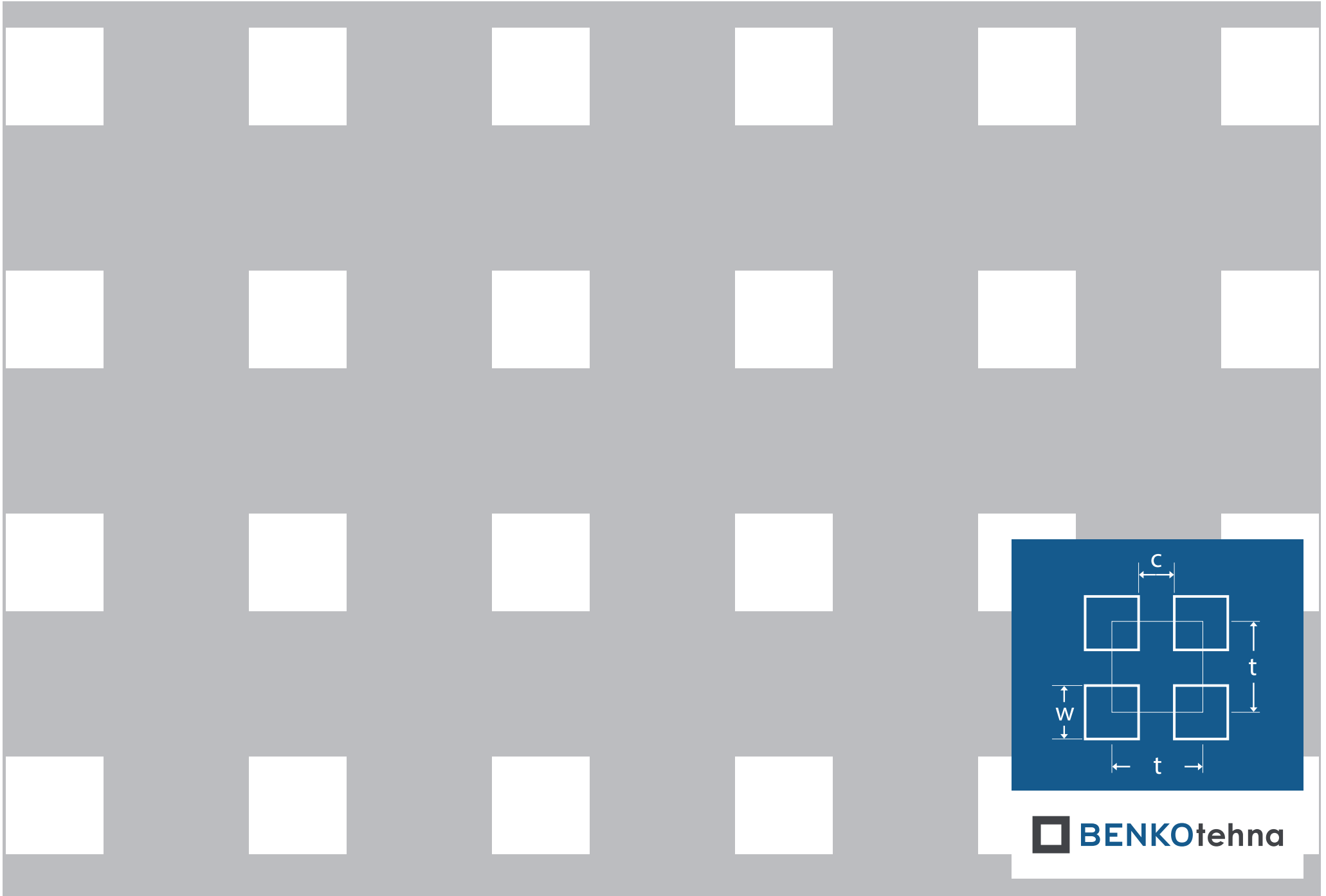
Kvadratna redna Kr 20-50: w = 20,0 \text{ mm} | c = 30,0 \text{ mm} | t = 50,0 \text{ mm} | otvorenost = 16,0%
