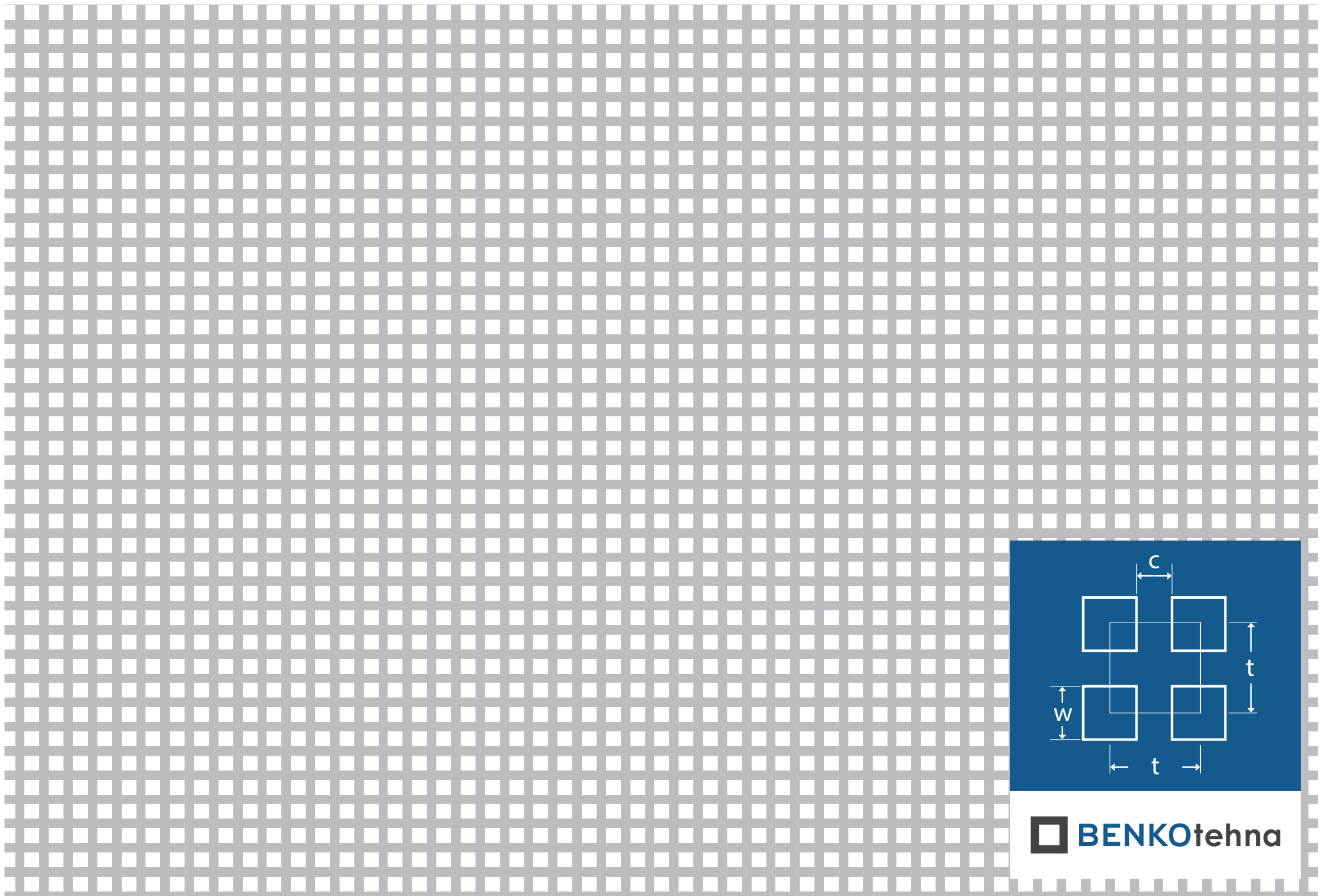
Kvadratna redna Kr 3-5: w = 3,0 \text{ mm} | c = 2,0 \text{ mm} | t = 5,0 \text{ mm} | otvorenost = 36,0%
