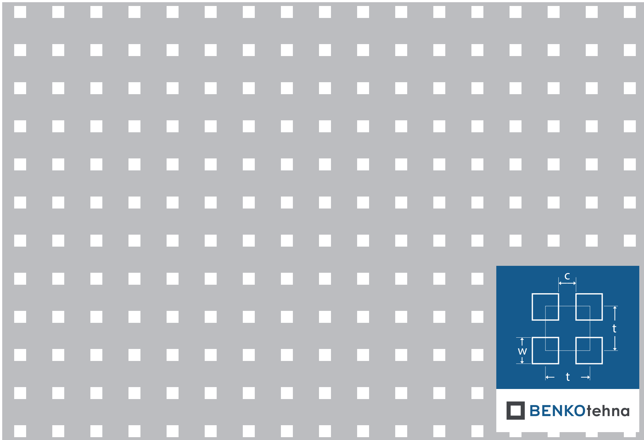
Kvadratna redna Kr 5-16: w = 5,0 \text{ mm} | c = 11,0 \text{ mm} | t = 16,0 \text{ mm} | otvorenost = 9,77%
