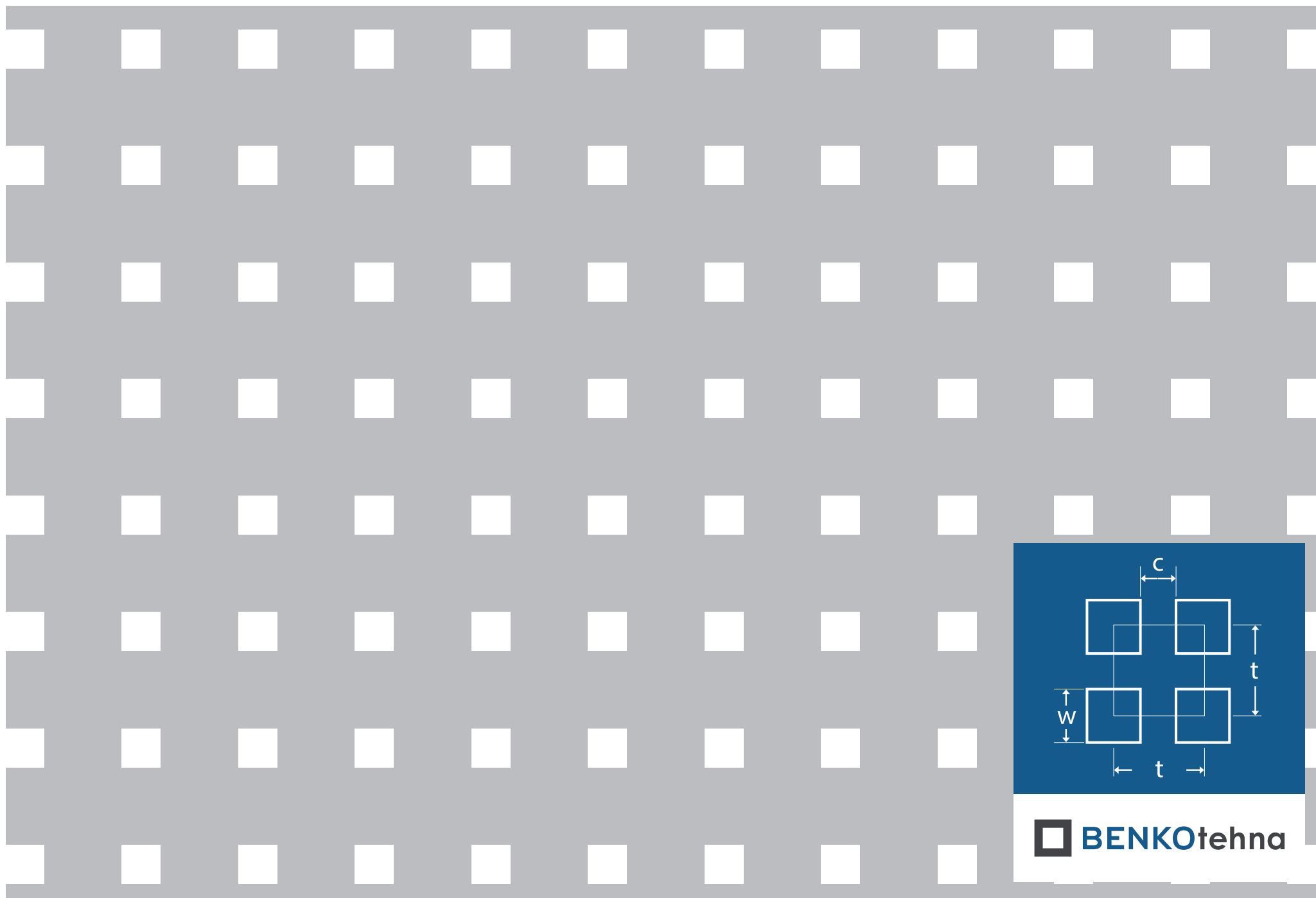
Kvadratna redna Kr 8-24: w = 8,0 \text{ mm} | c = 16,0 \text{ mm} | t = 24,0 \text{ mm} | otvorenost = 11,11%
