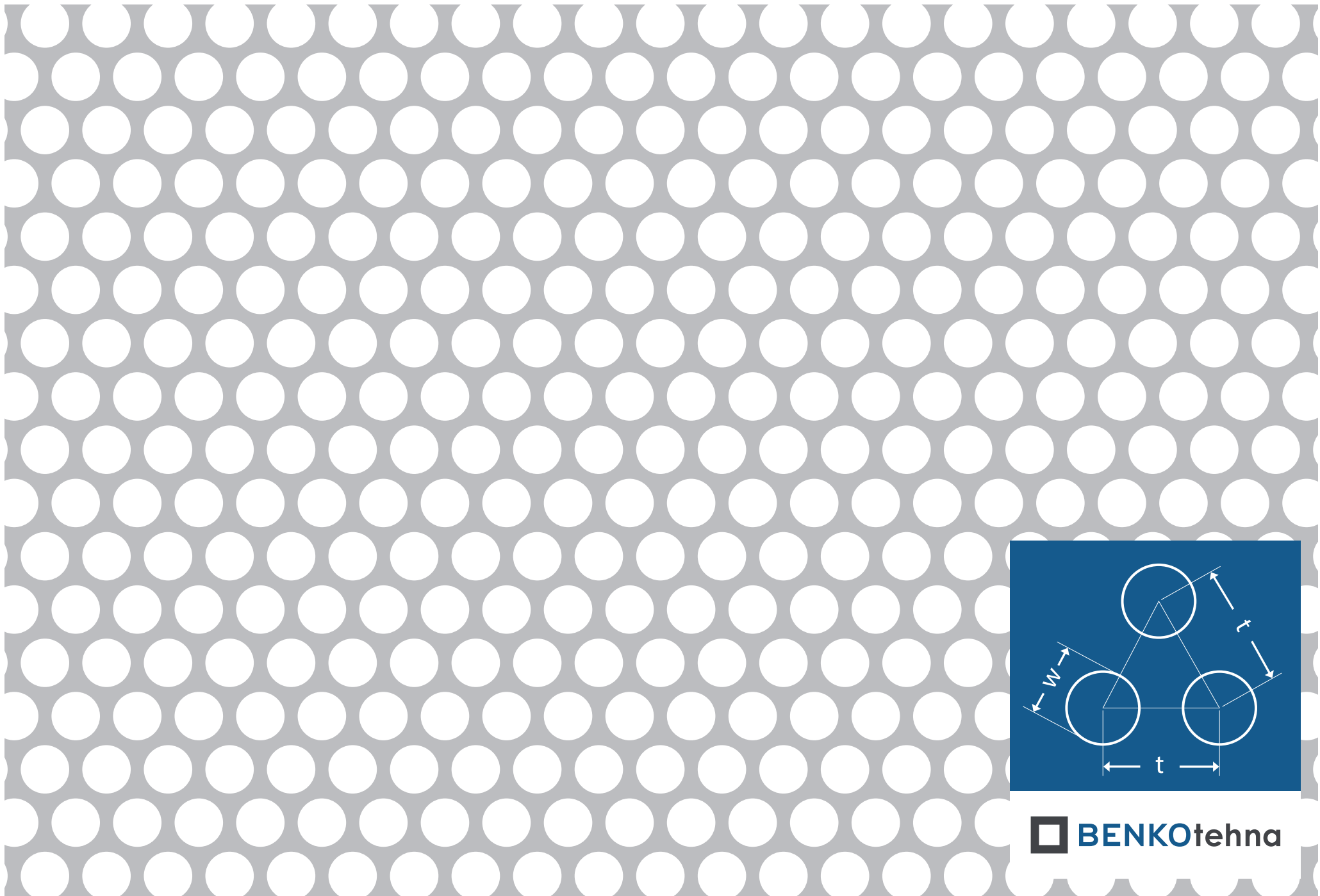
Okrugla s pomakom Op10-13: w = 10,0 \text{ mm} | t = 13,0 \text{ mm} | otvorenost = 53,67%
