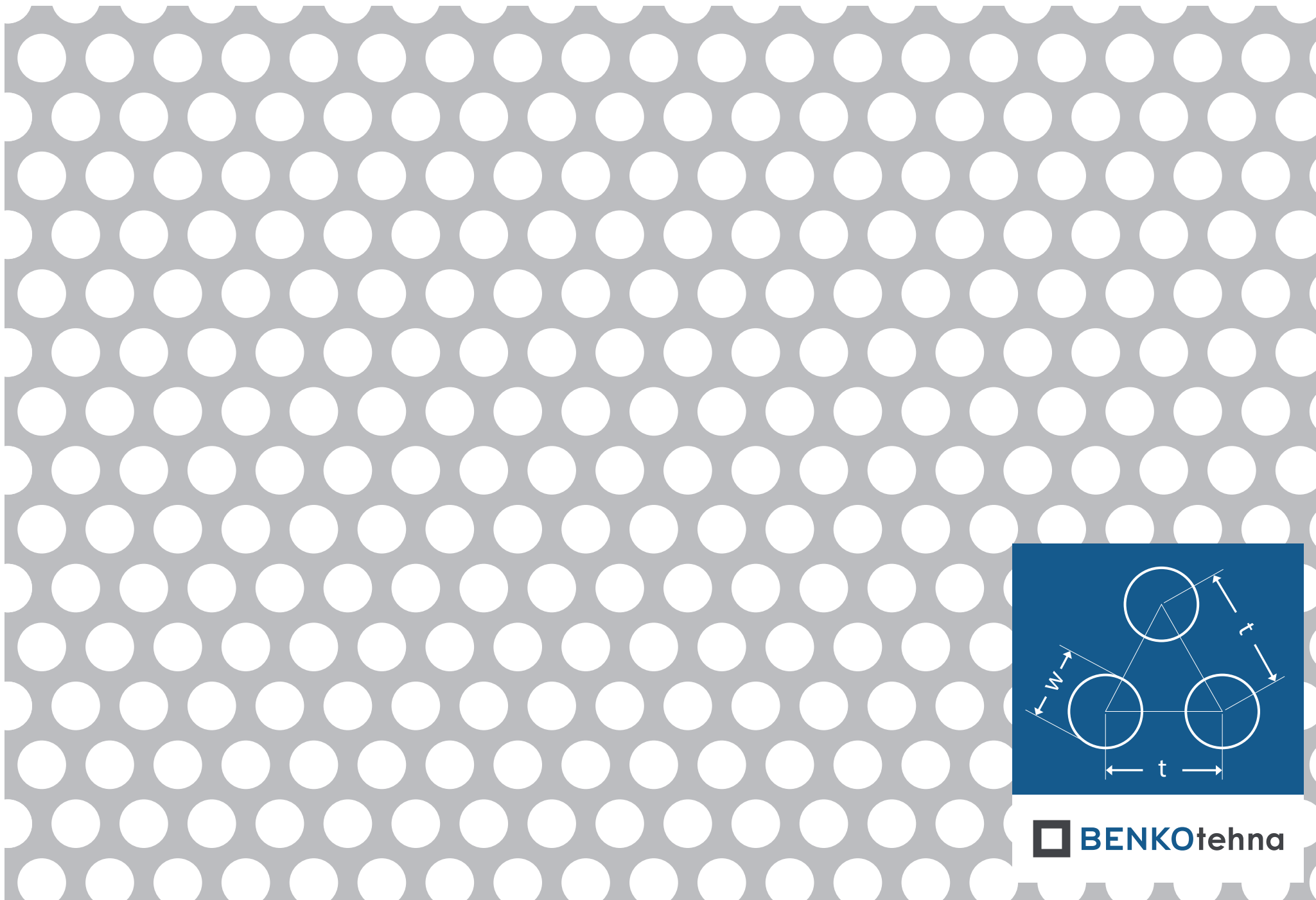
Okrugla s pomakom Op 10-14: w = 10,0 \text{ mm} | t = 14,0 \text{ mm} | otvorenost = 46,28%
