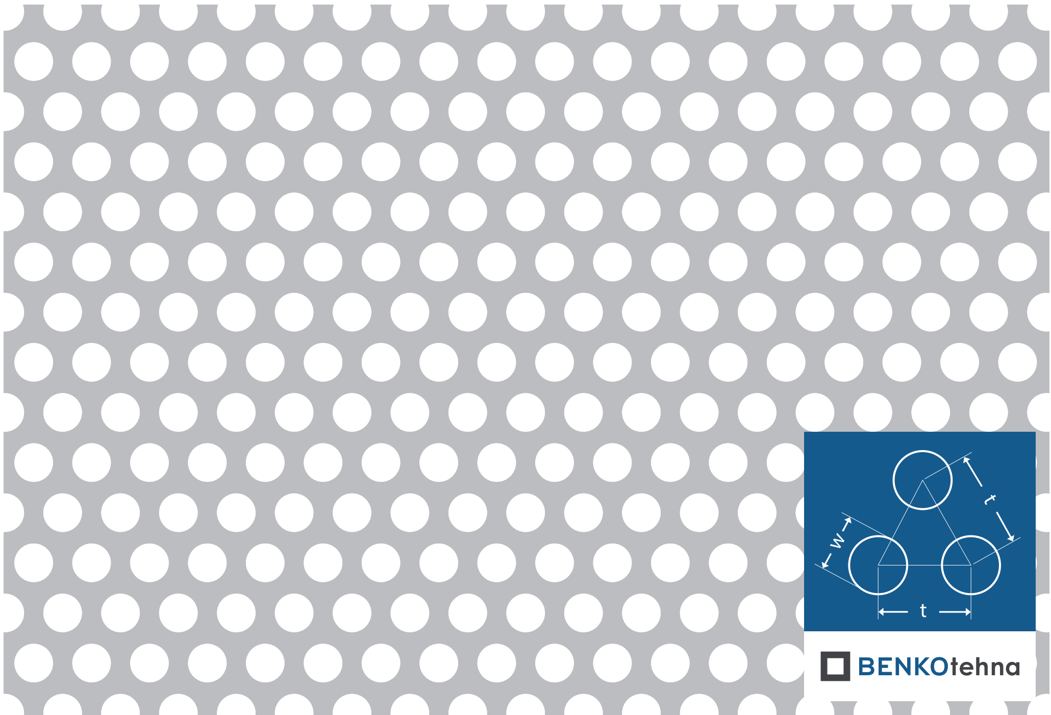
Okrugla s pomakom Op10-15: w = 10,0 \text{ mm} | t = 15,0 \text{ mm} | otvorenost = 40,31%
