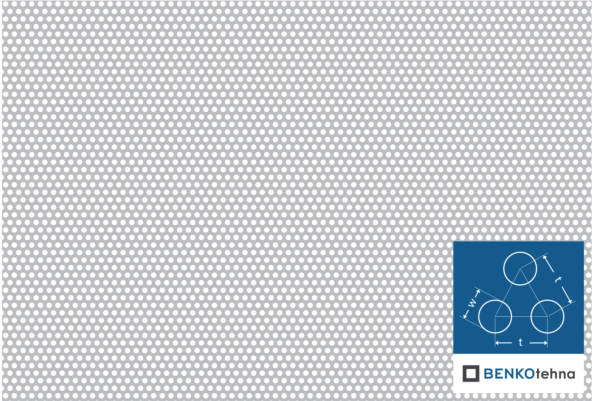
Okrugla s pomakom Op 2,5-4: w = 2,5 \text{ mm} | t = 4,0 \text{ mm} | otvorenost = 35,43%
