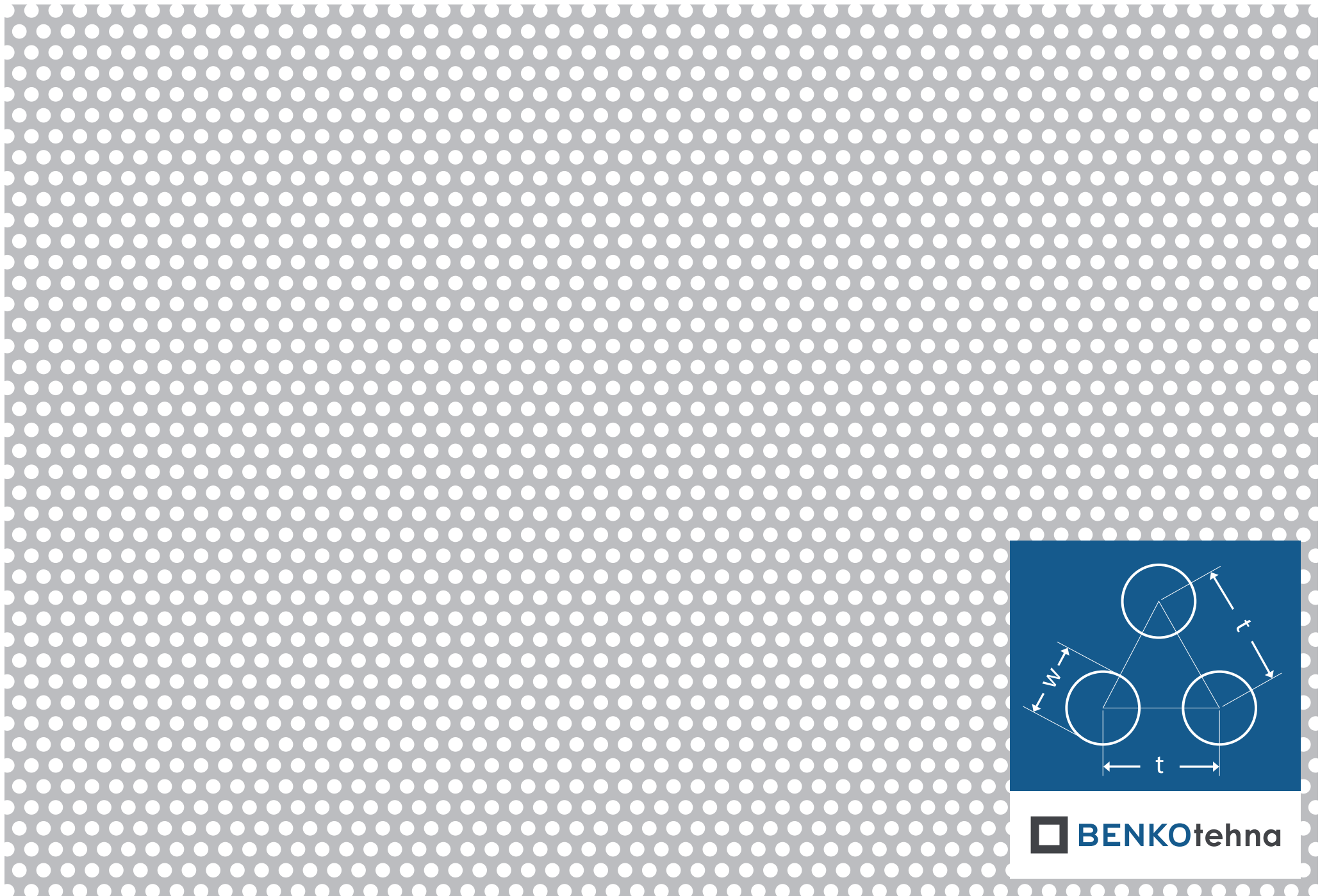
Okrugla s pomakom Op 3-5: w = 3,0 \text{ mm} | t = 5,0 \text{ mm} | otvorenost = 32,65%
