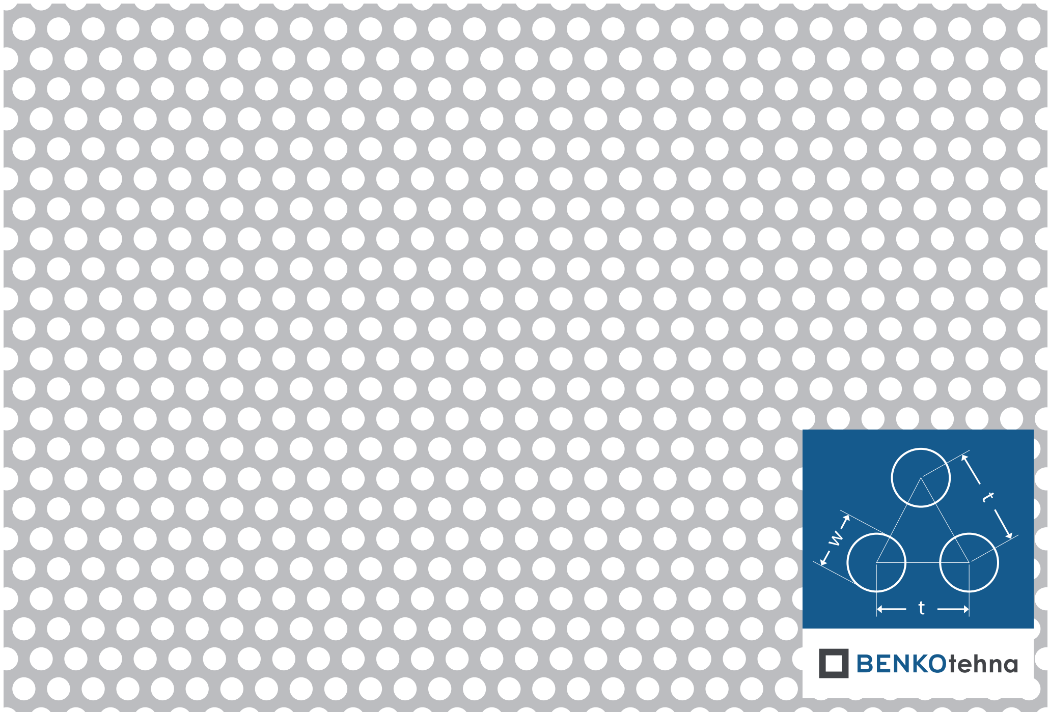
Okrugla s pomakom Op 6-9: w = 6,0 \text{ mm} | t = 9,0 \text{ mm} | otvorenost = 40,31%
