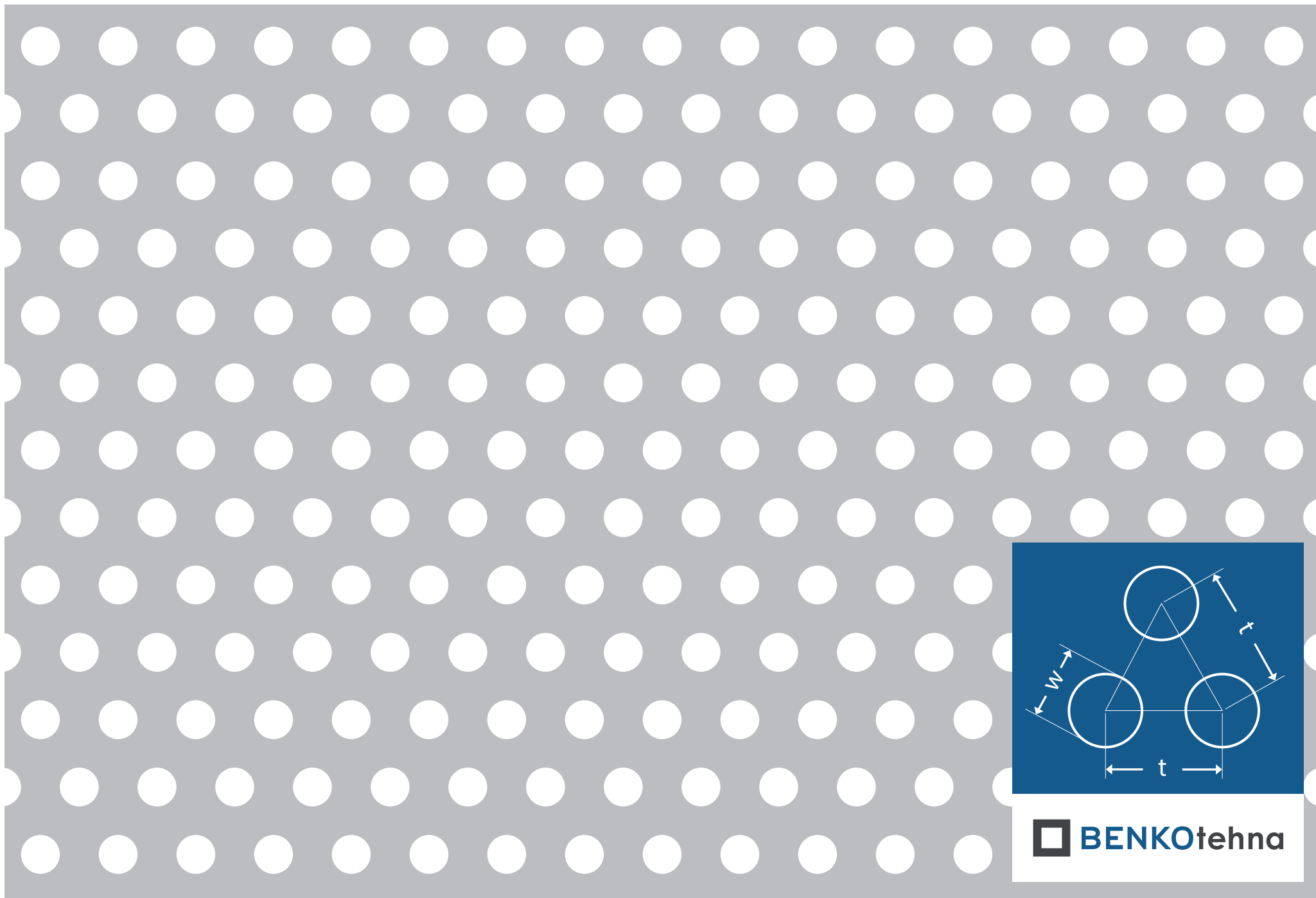
Okrugla s pomakom Op 8-16: w = 8,0 \text{ mm} | t = 16,0 \text{ mm} | otvorenost = 22,68%
