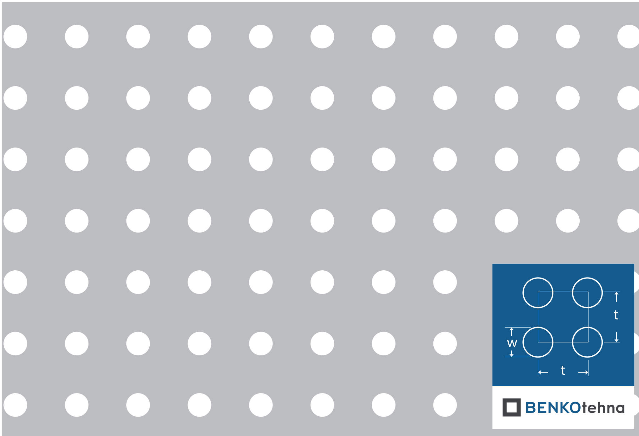
Okrugla redna Or 10-25,98: w = 10,0 \text{ mm} | t = 25,98 \text{ mm} | otvorenost = 11,63%
