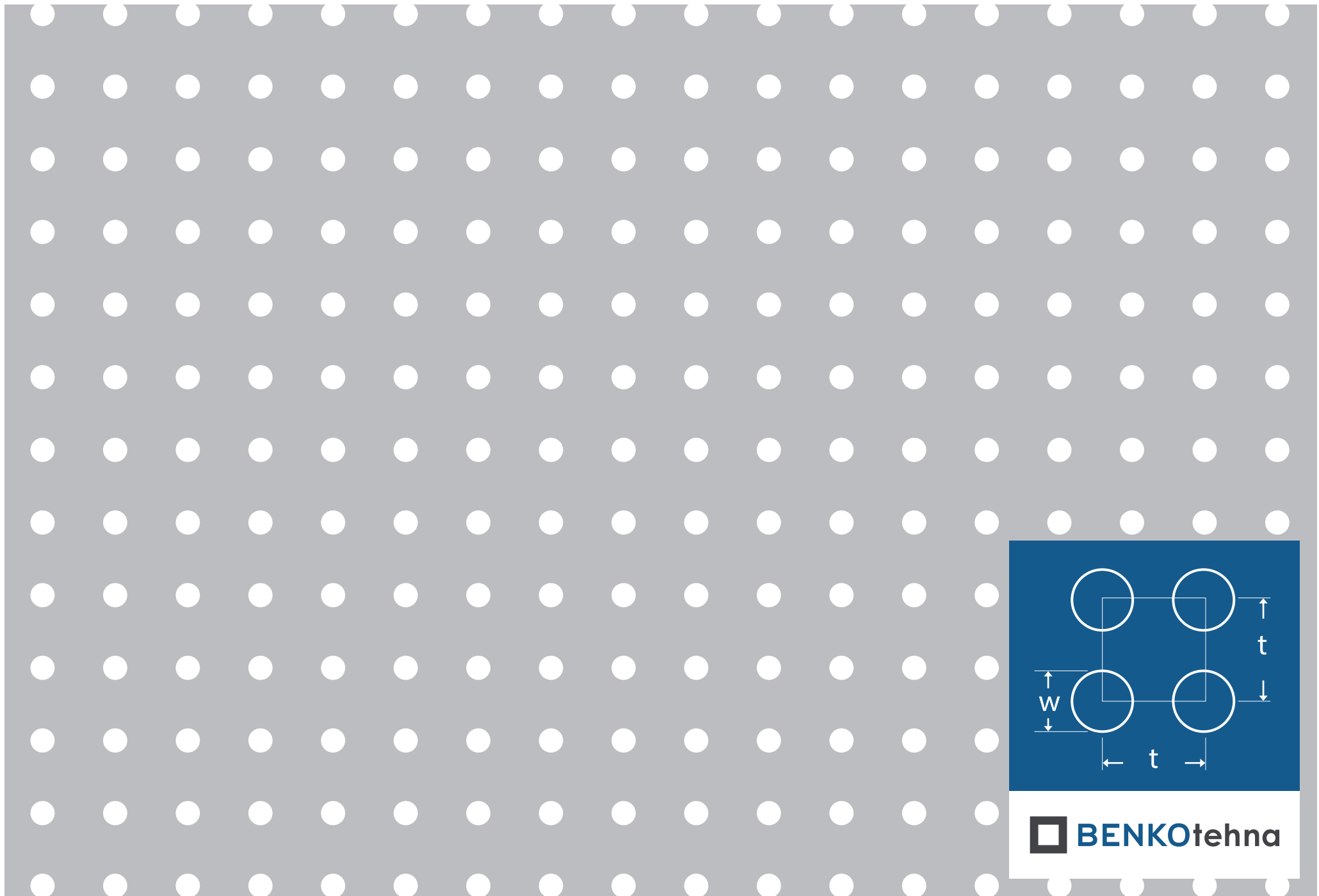
Okrugla redna Or 5-15: w = 5,0 \text{ mm} | t = 15,0 \text{ mm} | otvorenost = 8,72%
