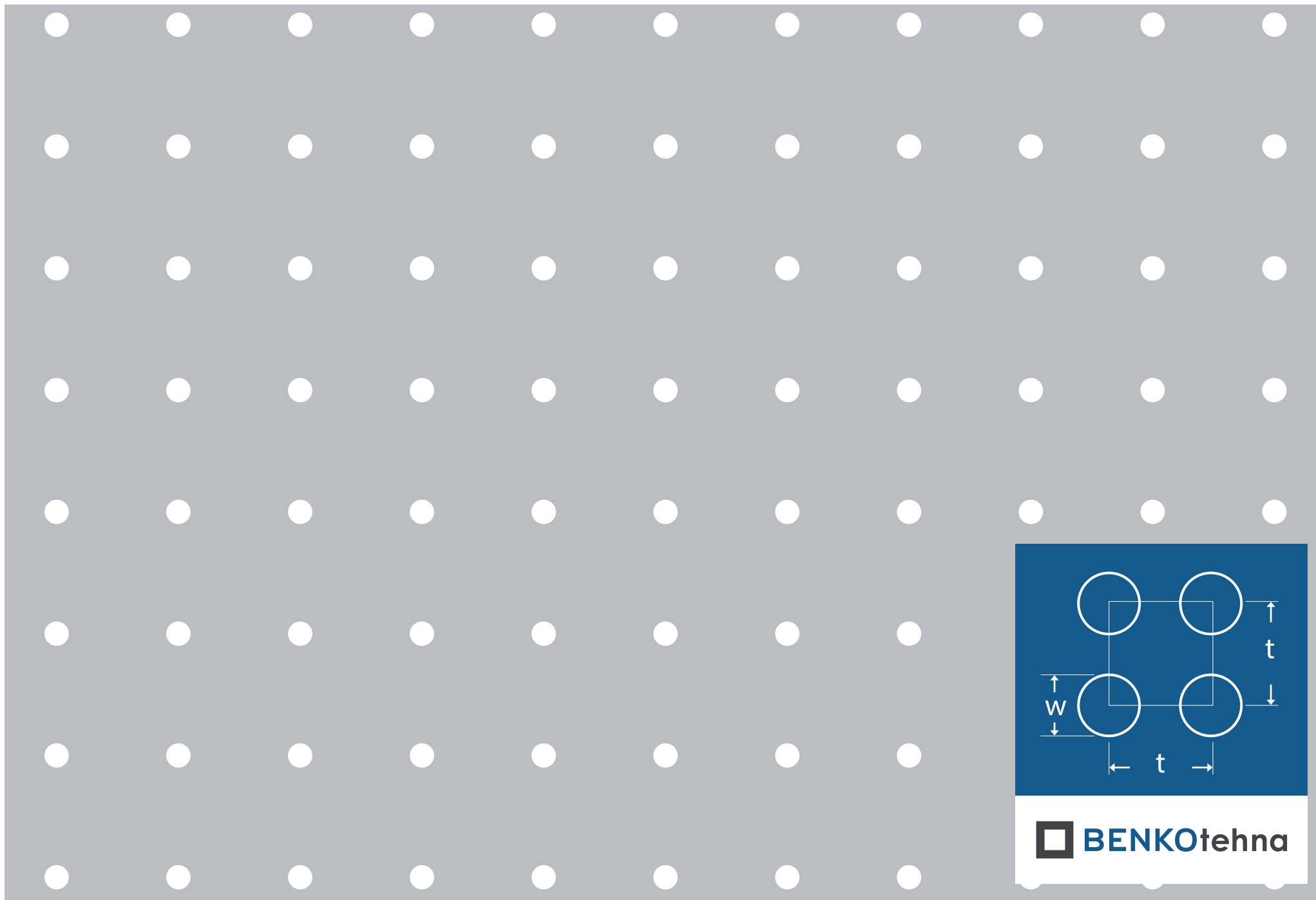
Okrugla redna Or 5-25: w = 5,0 \text{ mm} | t = 25,0 \text{ mm} | otvorenost = 3,14%
