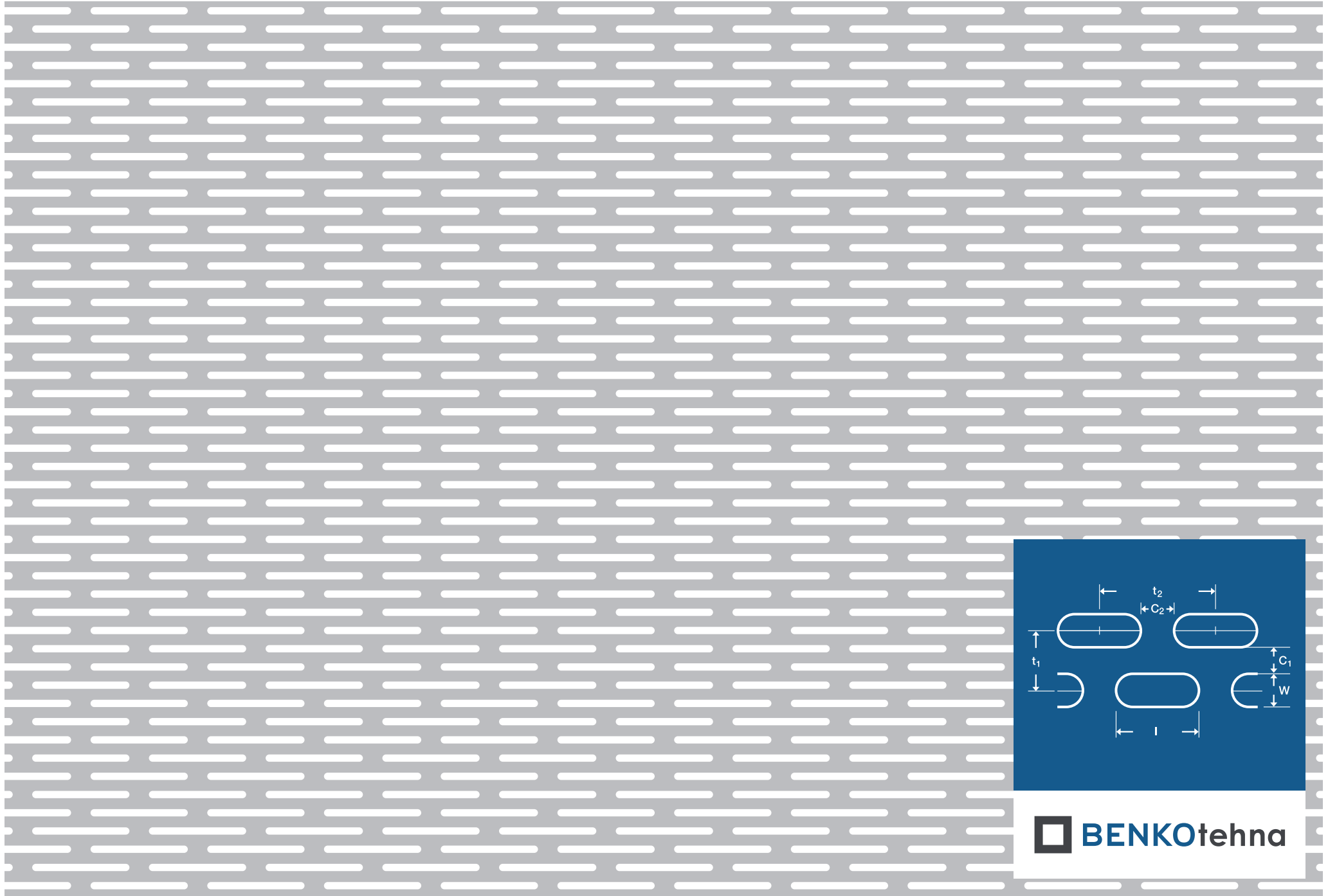
Uzdužna s pomakom Up 1,5×20 - 3,75×24: w = 1,5 \text{ mm} | c_1 = 2,25 \text{ mm} | c_2 = 4,0 \text{ mm} | t_1 = 3,75 \text{ mm} | t_2 = 24,0 \text{ mm} | l = 20,0 \text{ mm} | otvorenost = 31,8%
